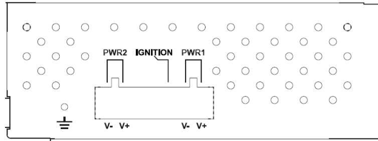
Top panel of the Industrial Switch Converter
